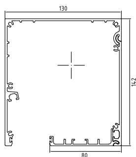
KASSETT 130 COMPACT
